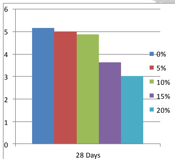
Graph No 2. Flexural strength test for M30 grade concrete
