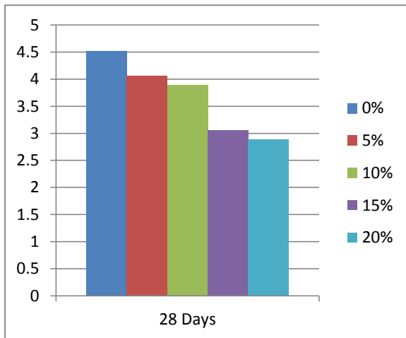
Graph No 1. Flexural strength test for M20 grade concrete
