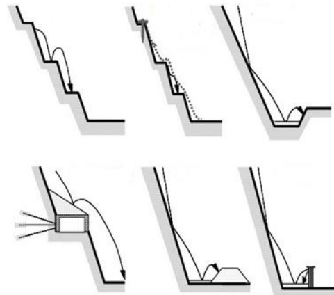
Figure 5: Road side cutting development
