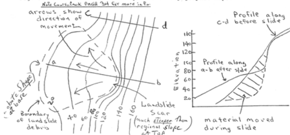
Figure 1: Landslides and mass movements contour study
